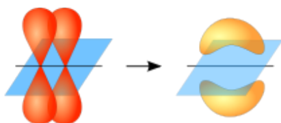
Two p-orbitals forming a ( \pi bond).
