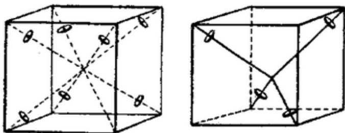
Fig. 4.10. Landé's cubical atom with the electrons moving in small circles near the corners of a cube. Source: Landé 1920, p. 382.
